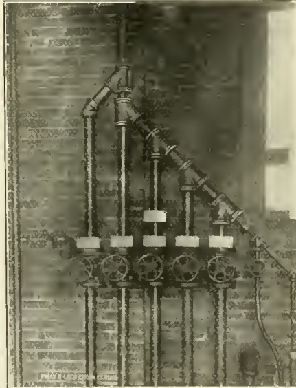
FIG. 2. "MANIFOLD" PIPE ARRANGEMENT FOR WATER CHANGING APPARATUS.
